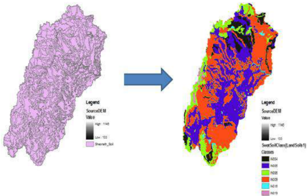
Fig. 4. Soil Map Reclassification in HRU Analysis
