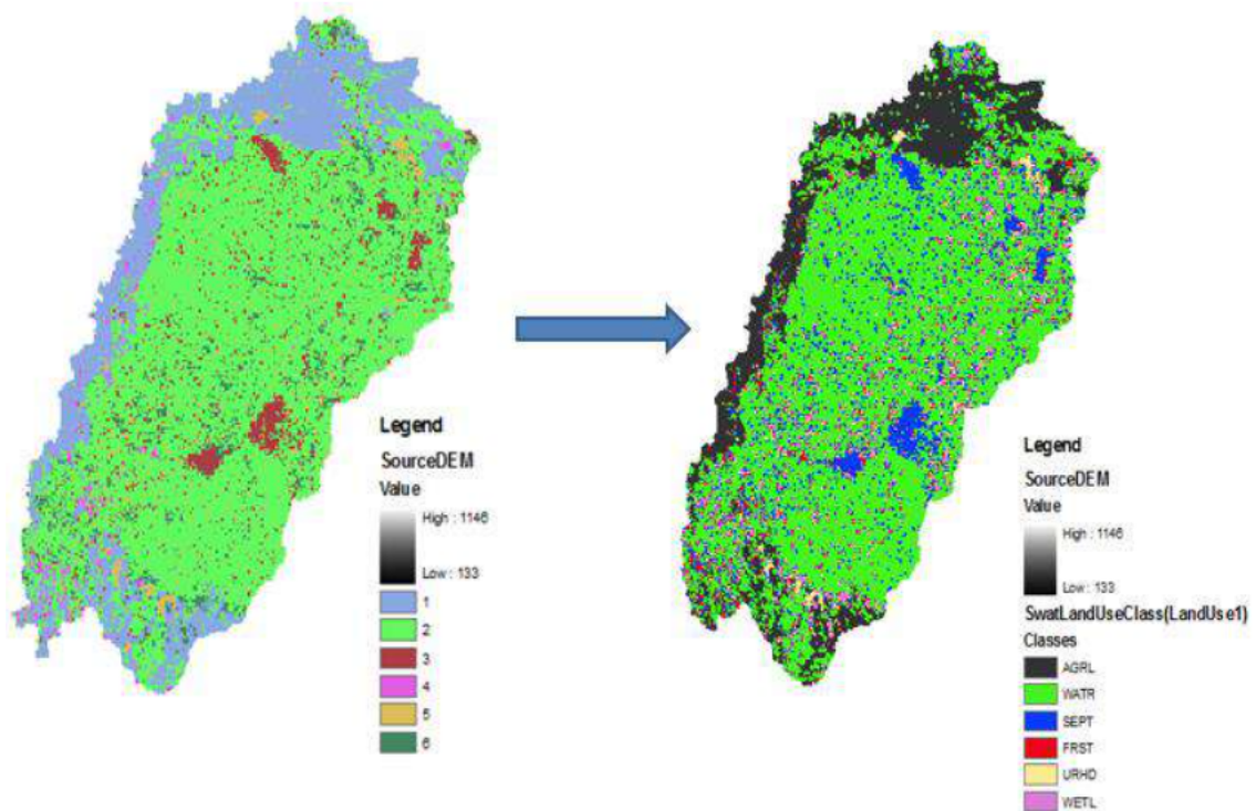
Fig. 3. LULC Map Reclassification in HRU Analysis
