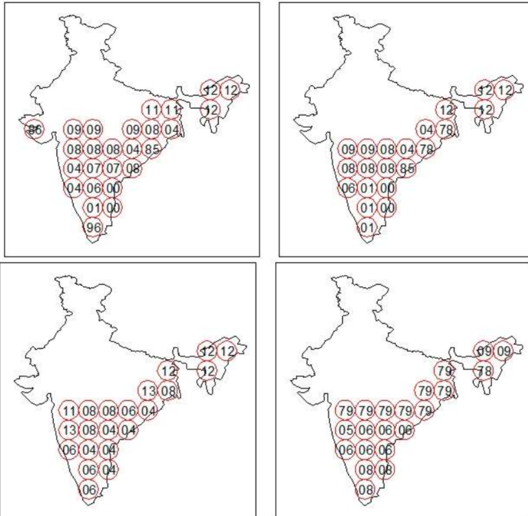
Fig. 4: Significant change points (Year) in monthly mean temperature during the south-west monsoon season estimated using Pettit's test (Clockwise from left top: Level Surface, Level 1000, Level 500, Level 850)
