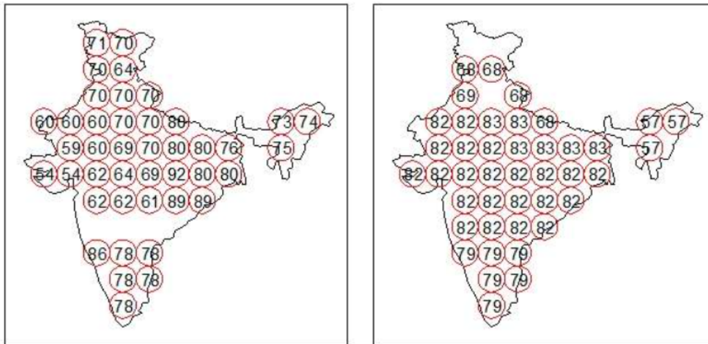
Fig. 5: Significant change points (Year) in annual mean temperature (excluding 2000-2014) estimated using Pettit's test (Clockwise from left top: Level Surface, Level 1000, Level 500, Level 850)
